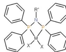
Scheme 1 General structure of the studied complexes [\text{M}(\text{P,P})\text{X}_2] , \text{M} = \text{Ni}, \text{Pd}, \text{Pt} ; \text{X} = \text{Cl}, \text{Br}, \text{I} ; \text{R}' = ((S)\text{-CHMePh}), (\text{CH}_2)_3\text{Si}(\text{OCH}_3)_3, \text{}^t\text{Bu} .
